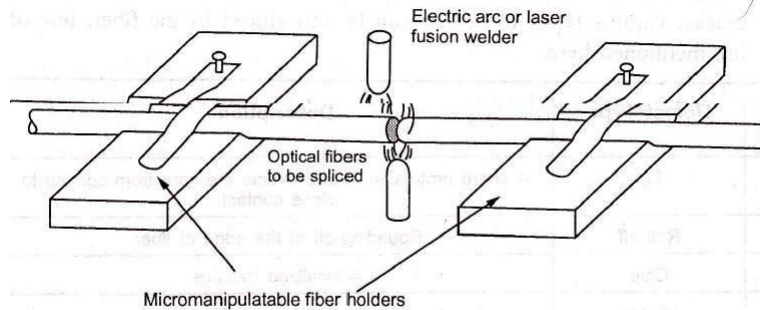
Fig. 4.2.1 Fusion splicing of optical fibers
