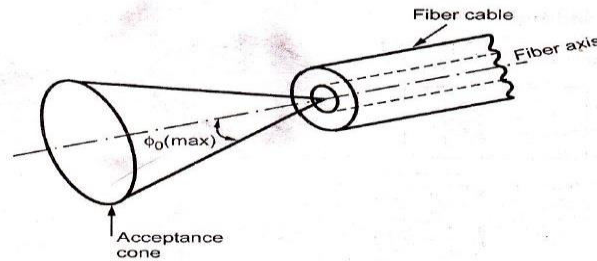
Fig. 1.6.10 Acceptance cone of a fiber cable
