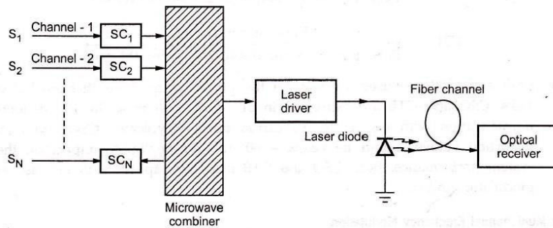
Fig. 6.1.5 Sub-carrier multiplexing
