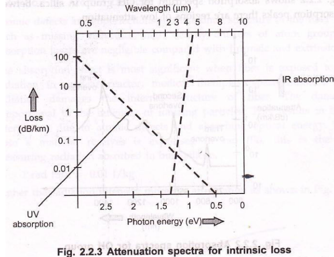
Fig. 2.2.3 Attenuation spectra for intrinsic loss
