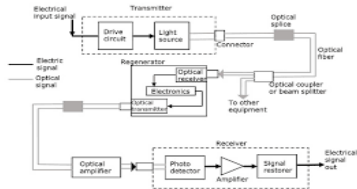
Fig. 1.2.1. General block diagram of optical fiber communication system
