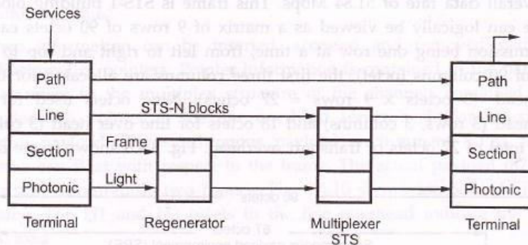
Fig. 8.4.7 (a) Logical hierarchy
