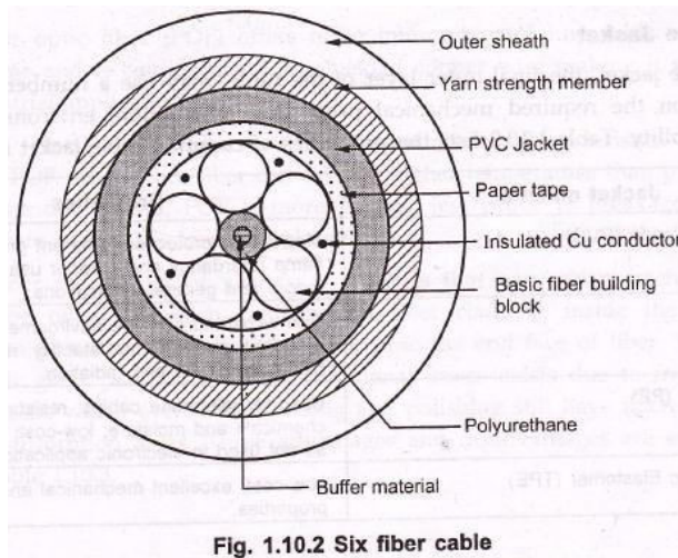
Fig. 1.10.2 Six fiber cable
