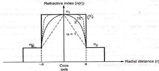
Fig. 1.6.15 Possible fiber refractive index profiles for different values of \alpha .
