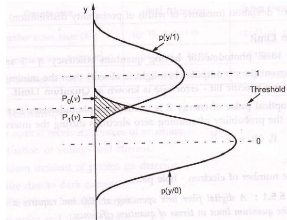
Fig. 5.5.1 Probability distribution of received 1 and 0
