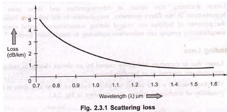
Fig. 2.3.1 Scattering loss
