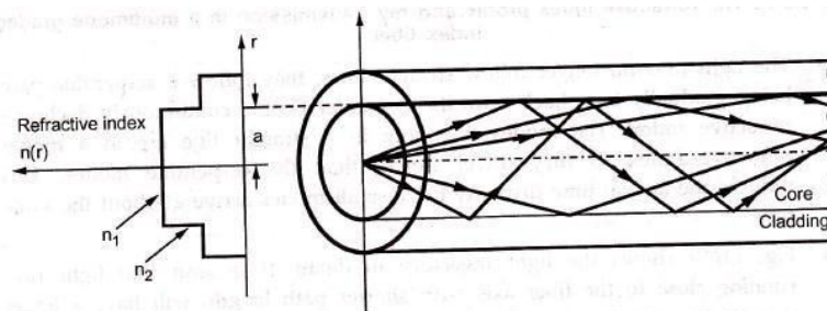
Fig. 1.6.17 TIR in multimode step index fiber
