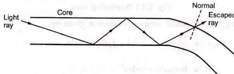
Fig. 2.4.1 Bending loss
