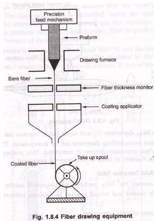
Fig. 1.8.4 Fiber drawing equipment
