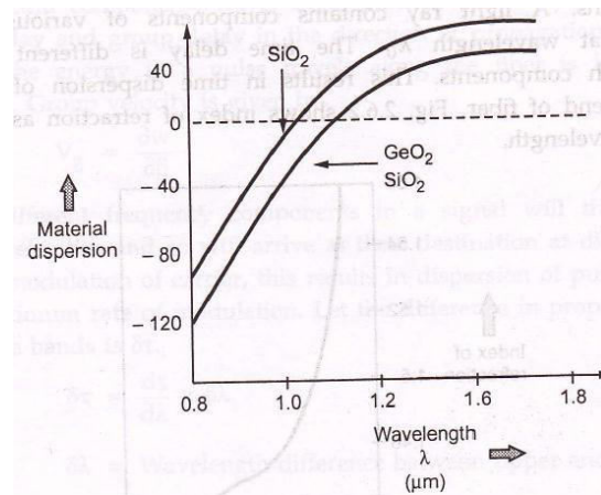
Fig. 2.6.3 Material dispersion as a function of \lambda
