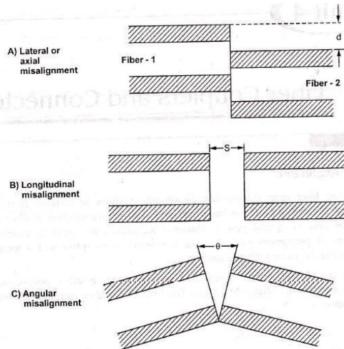
Fig. 4.1.1 Mechanical misalignment between two fibers
