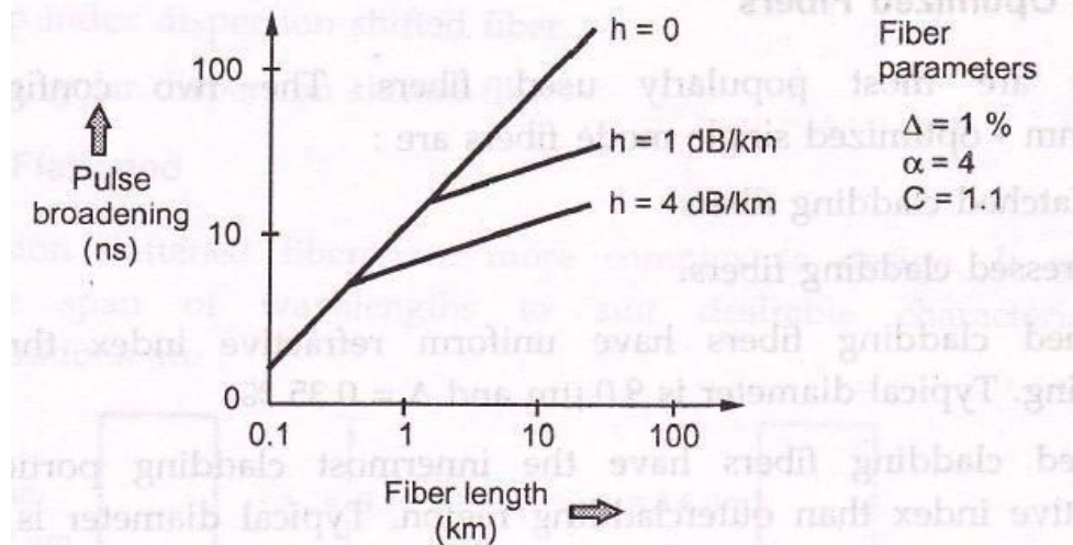
Fig. 2.8.1 Mode coupling effects on pulse broadening
