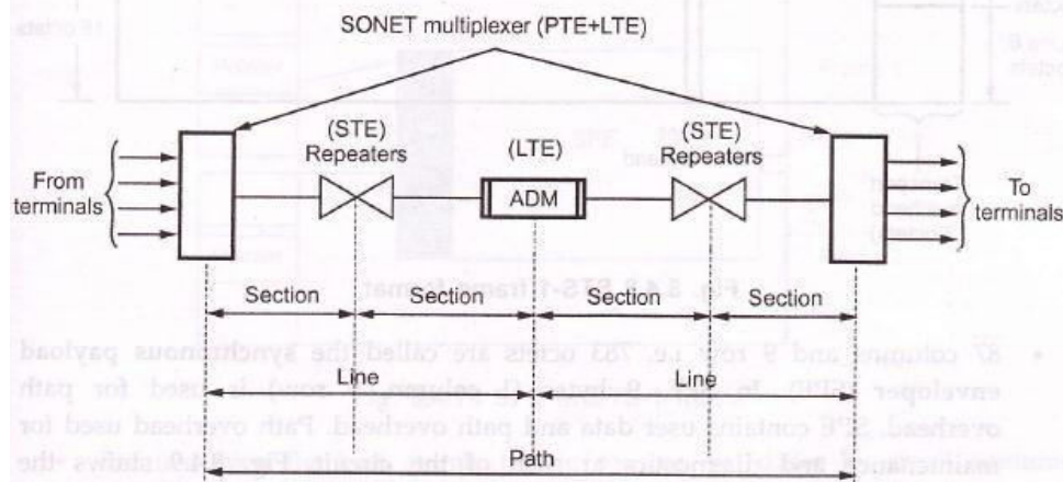
Fig. 8.4.7 (b) System hierarchy
