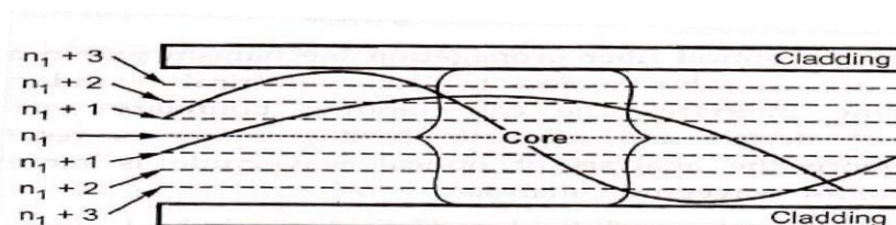
Fig. 1.6.19 Light trajectories in a graded index fiber
