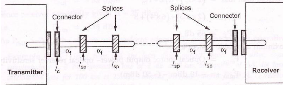
Fig. 6.2.3 Optical power loss model
