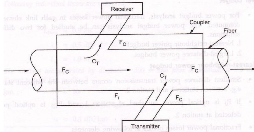
Fig. 7.1.5 Losses in bus coupler
